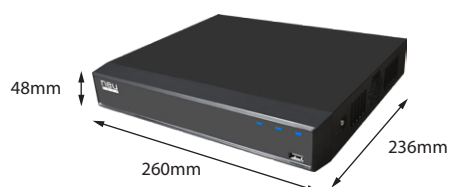
Dimensions (mm)
